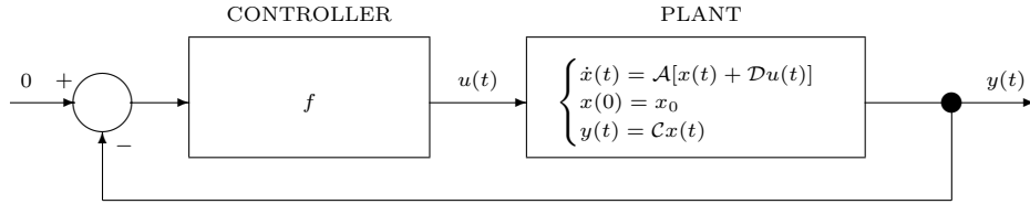
Fig. 1. The Lur'e control system with negative feedback
