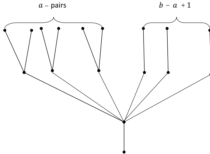
Fig. 5. A graph G with c(\mathcal{M}_G) = r
