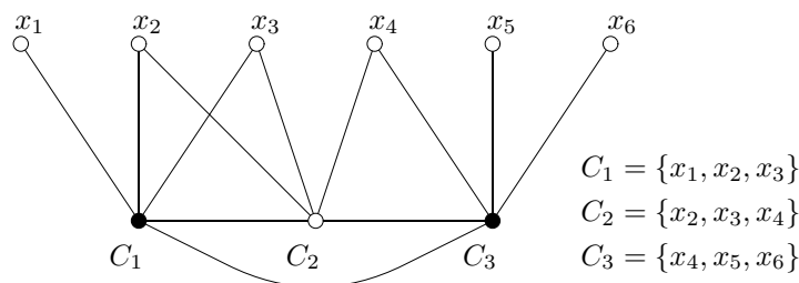
Fig. 1. Split graph
