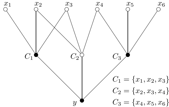
Fig. 2. Bipartite graph
